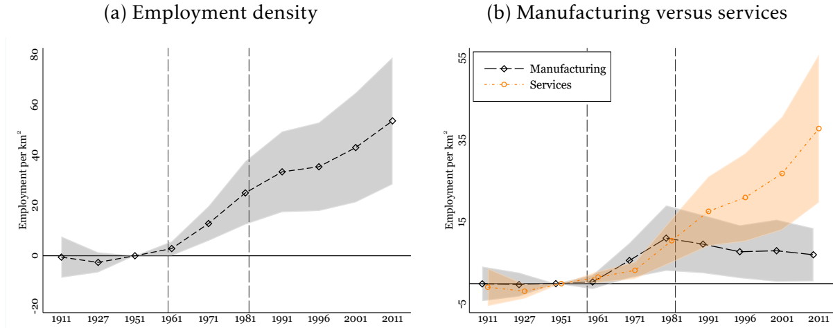
Figure 6. Difference-in-discontinuities
